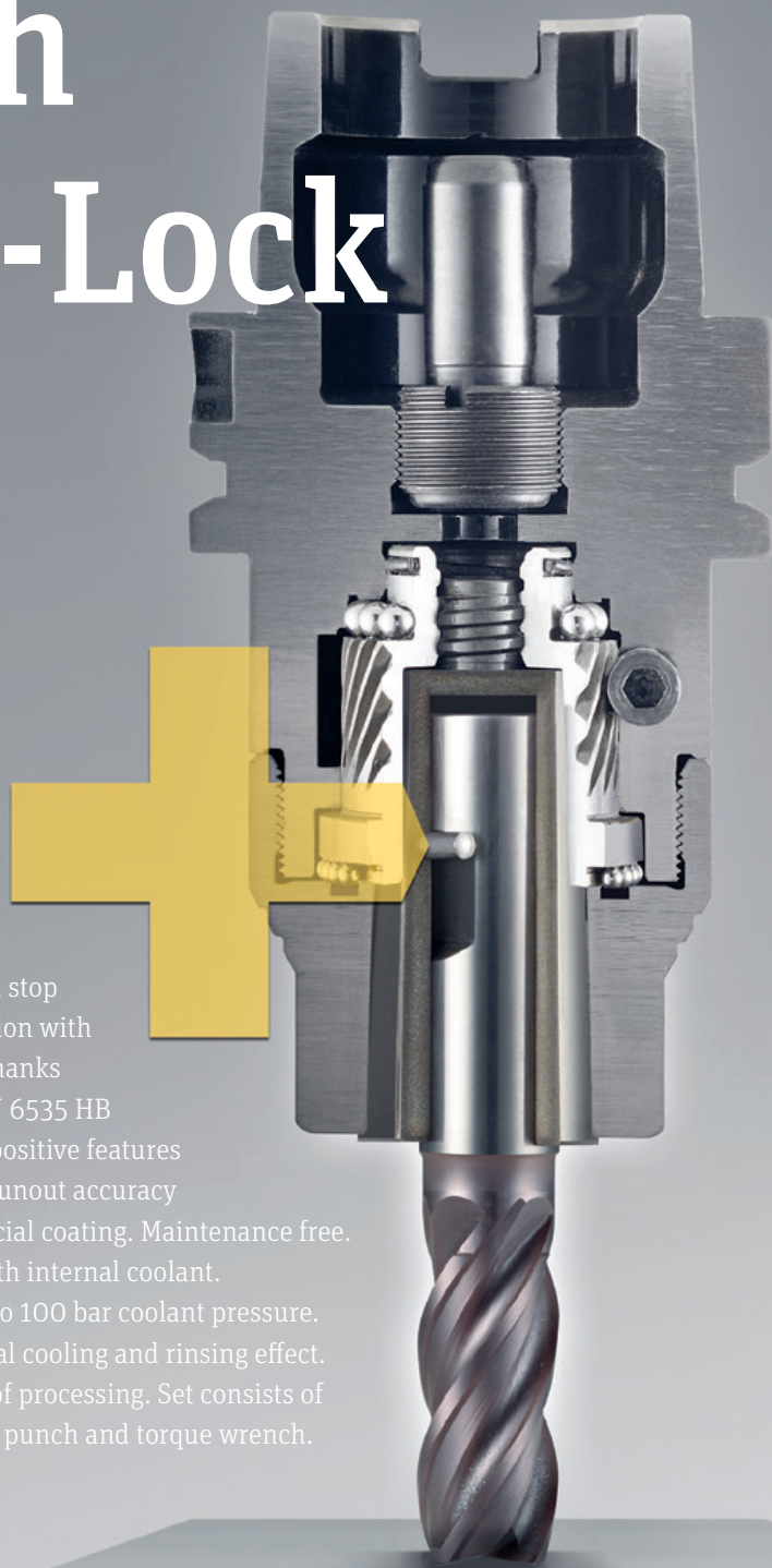
APC collet with mechanical pull stop Pin-Lock
